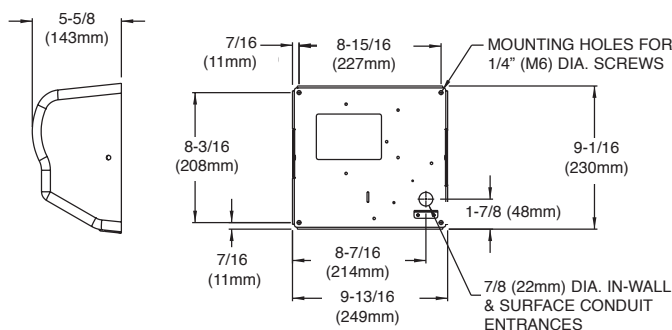
Figure 1 - EXT Series Surface Mount
